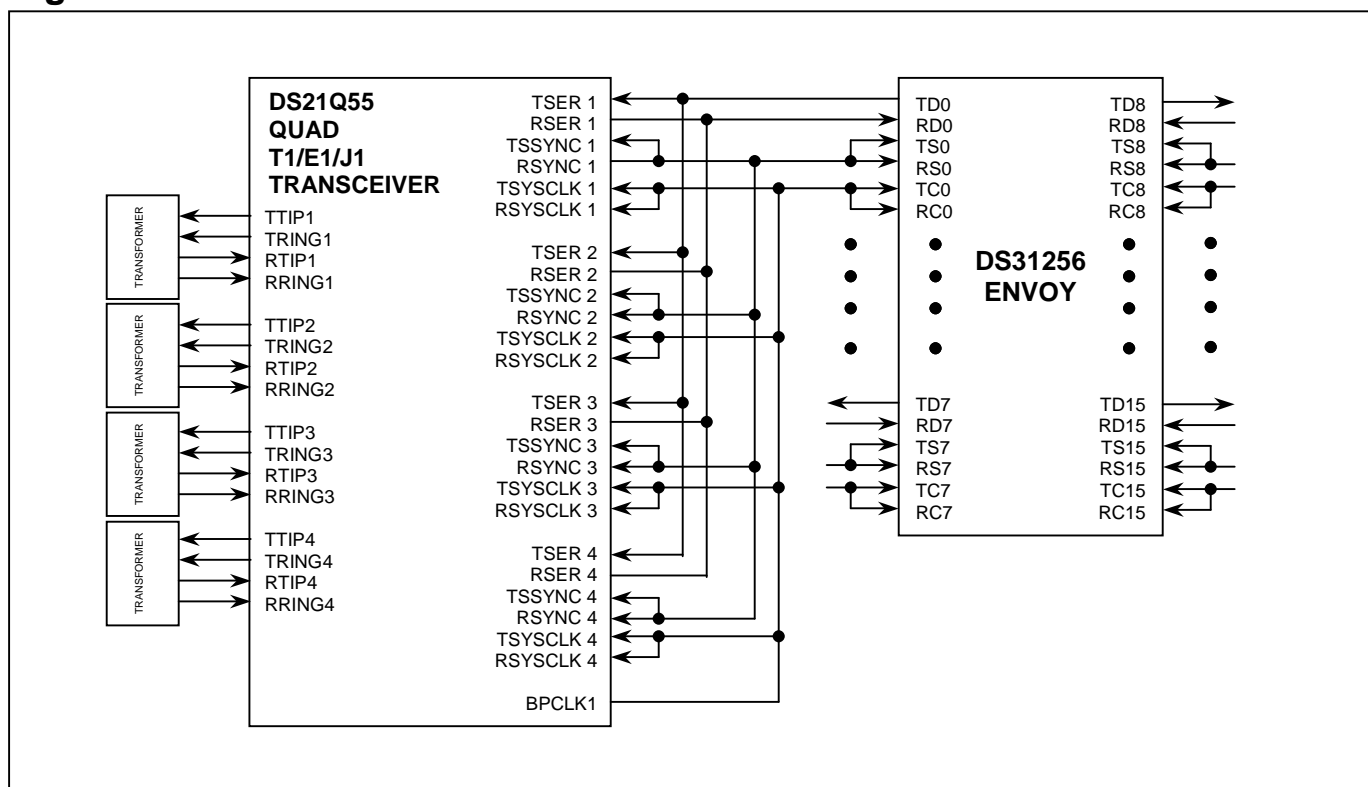
Figure 3. DS21Q55 Connected to DS31256 in 8M Mode
