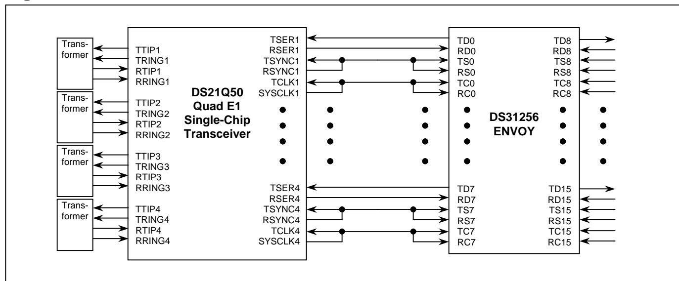
Figure 4. DS21Q50 Connected to DS31256 in 2M Mode
