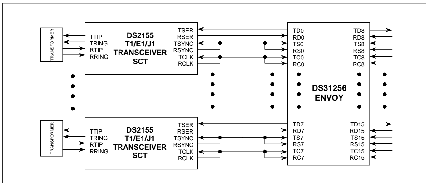
Figure 1. DS2155 Connected to DS31256 in T1 and E1 Mode
