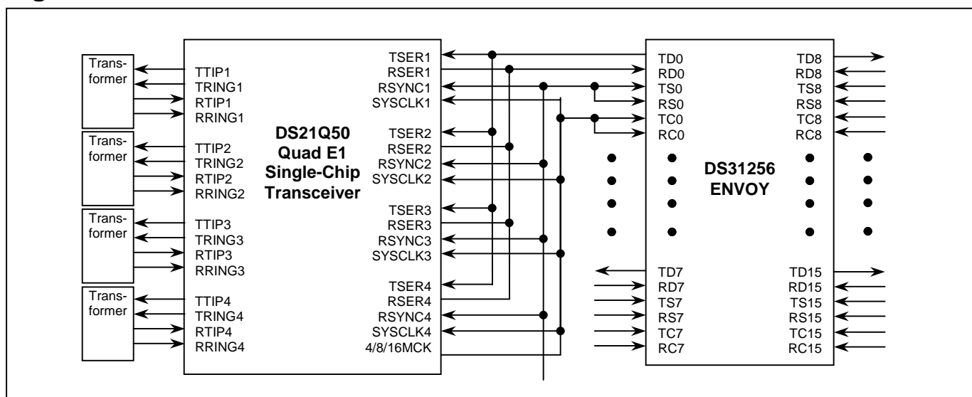
Figure 5. DS21Q50 Connected to DS31256 in 8M Mode
