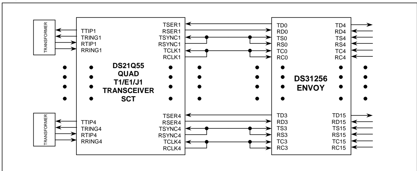
Figure 2. DS21Q55 Connected to DS31256 in T1 Mode
